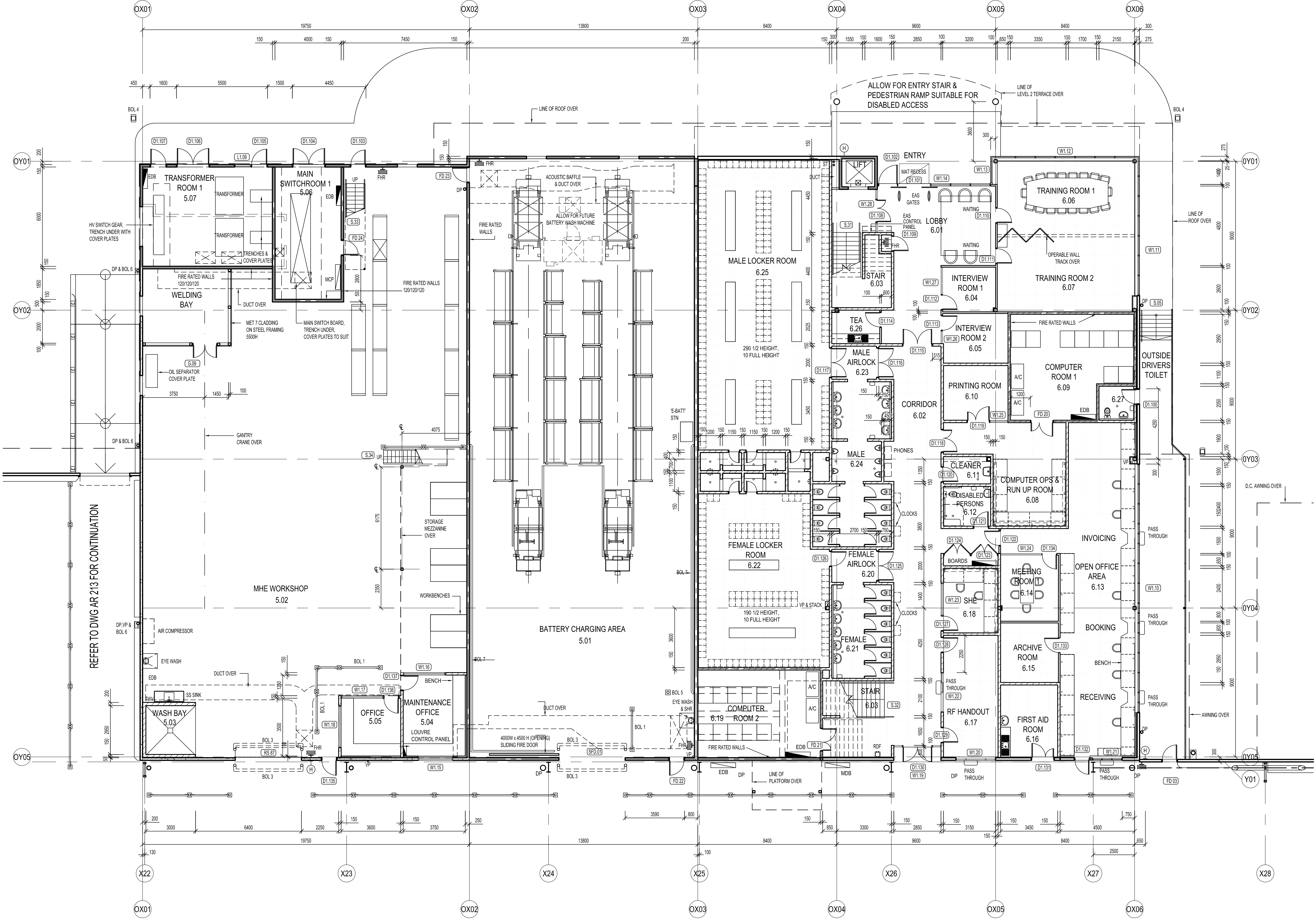
01 OFFICE AREA FLOOR PLAN LEVEL 1
